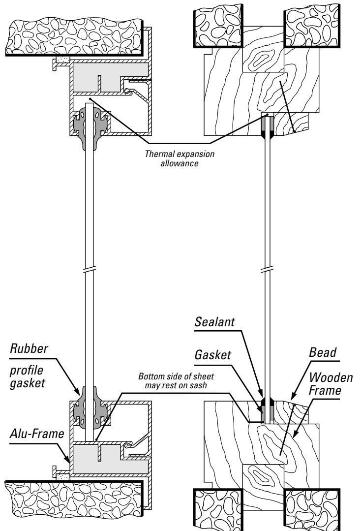
Dry glazing installation
