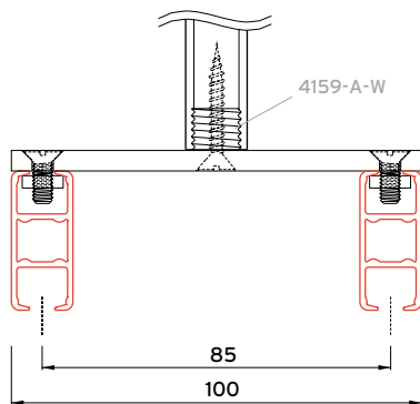
parallel rail fixing with bridging plate 4116-10
