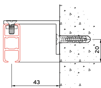
wall fixing with bracket 4141
