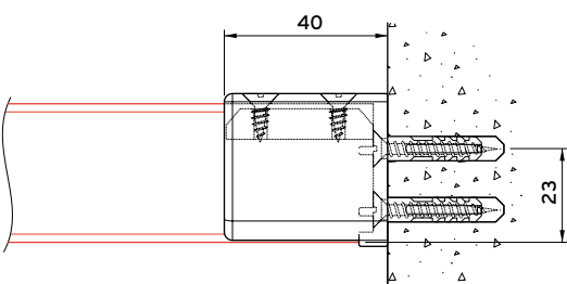
wall fixing with bracket 4150
