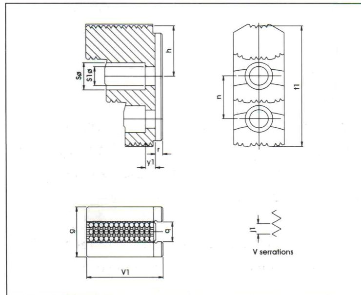
HARD JAW SPECIFICATIONS
